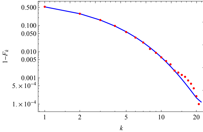
Fig. 5. Complementary cumulative degree distribution for a simulated network with \alpha = 0.3 (dotted curve) and the theoretical prediction (solid curve).
