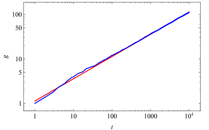
Fig. 4. Degree dynamics for a node that attaches to the network at t = 1 and the theoretical prediction.
