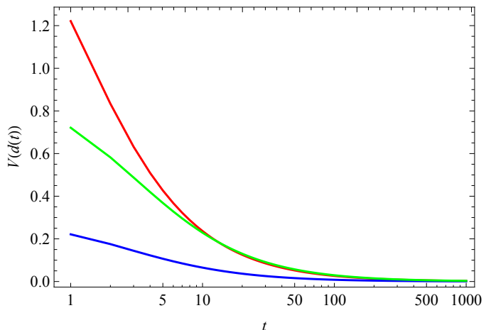
Fig. 8. Evolution of V for different initials networks.
