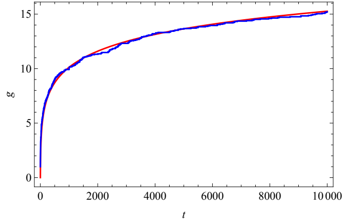
Fig. 3. Degree dynamics for a node that attaches to the network at t = 1 and the theoretical prediction.
