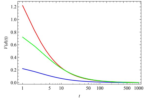
Fig. 8. Evolution of V for different initials networks.
