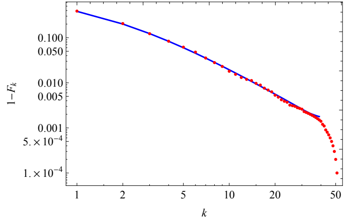
Fig. 6. Complementary cumulative degree distribution for a simulated network with \alpha = 1 (dotted curve) and the theoretical prediction (solid curve).
